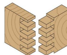
Box joint
